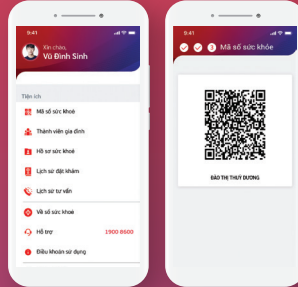
QR Android
